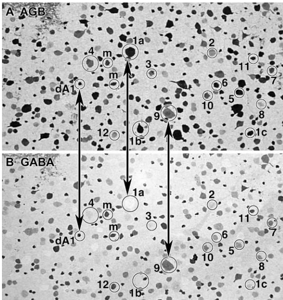
Fig. 4. Two images (A, AGB; B, GABA) from a 7-dimensional molecular series through the rabbit ganglion cell layer after activation with 25 μM AMPA. These two panels show correlated signals of 15 classes of resident neurons in the ganglion cell layer, including \gamma + displaced starburst amacrine cells (dA1) and 14 classes of ganglion cells. Two misplaced amacrine cells (m) are also indicated. Each image is 885 μm in width. Excerpted from Marc and Jones (2002) by permission of the Society for Neuroscience.
