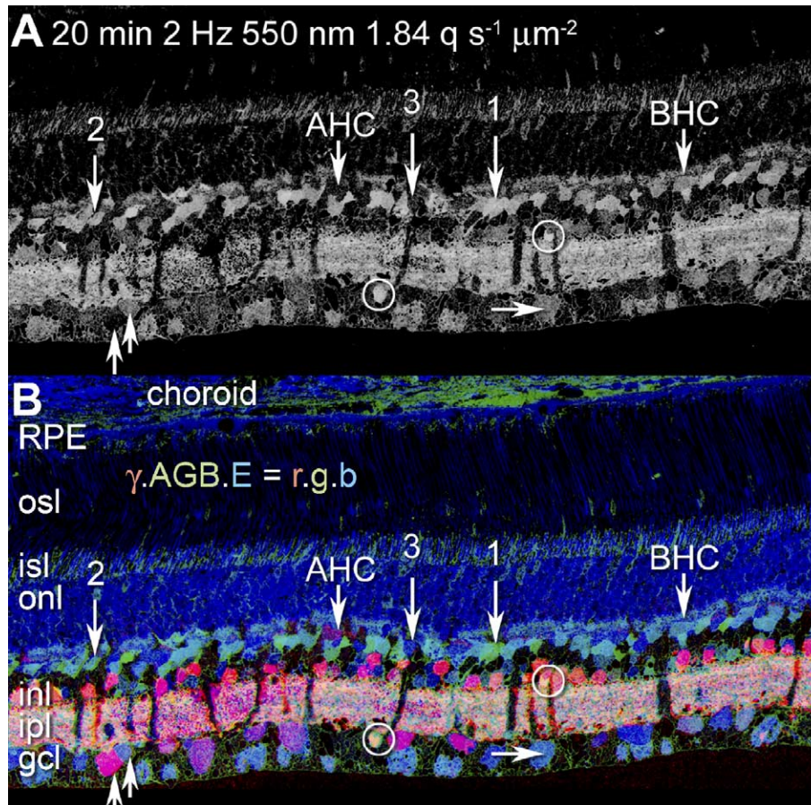
Fig. 9. Light-driven AGB signals in the in vitro rabbit retina with intact RPE and choroid. The retina was driven 20 min with 1.84 \text{ quanta s}^{-1} \mu\text{m}^{-2} 550 nm 2 Hz 2 -wave light (50% duty cycle) in Ames medium with 5 mM AGB. The top panel (A) shows the AGB response alone (as an inverted, brightness-scaled image) and the bottom (B) is a \gamma \cdot \text{AGB} \cdot E = \text{r.g.b} mapping. Strong permeation was activated in a great range of target neurons including all rod bipolar cells, cone OFF bipolar cells and most but not all cone ON bipolar cells and not type A horizontal cells. Cell classes were defined by CMP signatures (see Marc, 1999a; Marc and Jones, 2002). Arrows denote instances of the three modes of cone ON bipolar cell responses. Mode 1 is a highly responsive cohort, mode 2 shows moderate responses and mode 3 shows no responses. ON and OFF starburst amacrine cells are circled, which have strong mesopic light responses. Ganglion cell signals were weaker and varied by class (upward arrows) with \alpha -like cells (horizontal arrows) showing mid-range responses.
