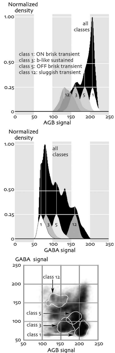
Fig. 5. Peak-normalized AGB and GABA univariate and bivariate signal strength histograms for a sample of over 600 ganglion cells. The abscissa is the 8-bit AGB or GABA grey level intensity (0–255) and the ordinate is normalized probability density. Top: the histogram for all cells in the ganglion cell layer is shown in black. The underlying histograms for classes 1, 3, 5, and 12 (see Fig. 4) are arbitrarily normalized to 0.25 to visualize their different positions along the AGB signal axis. Class 1 cells are the most AMPA-responsive. Middle: the same sets of cells visualized as histograms of GABA signals. Bottom: the same sets of cells visualized as a bivariate AGB vs GABA density histogram with the borders of the 95% level skirts of each class outlined in white. Bivariate clustering shows better separability than univariate analysis.
