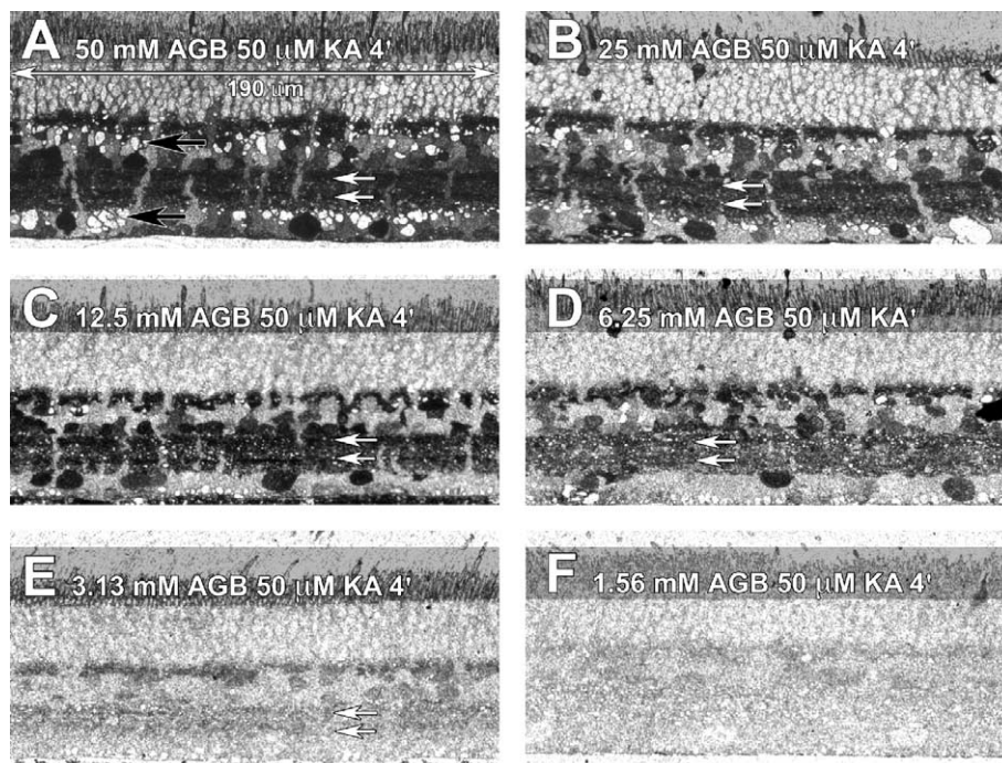
Fig. 7. The concentration-dependence of AGB permeation. A single rabbit retina was cut into chips and each concurrently incubated for 4 min in 50 \mu M KA and serial 2-fold dilutions of AGB ranging from 50 to 1.56 mM (A–F). As in Fig. 6, white arrows mark the starburst amacrine strata. This sample showed some Müller cell swelling at the highest concentrations, but this is a variable effect and may be due to mechanical stimulation (see Marc, 1999b).
